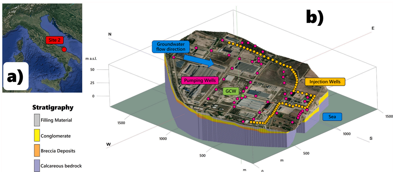
Fig. 2. Geographical location of Site 2 on the Italian peninsula (a) and a 3D stratigraphic model of the site indicating the position of the industrial plant's pumping wells and the direction of groundwater flow (b).
